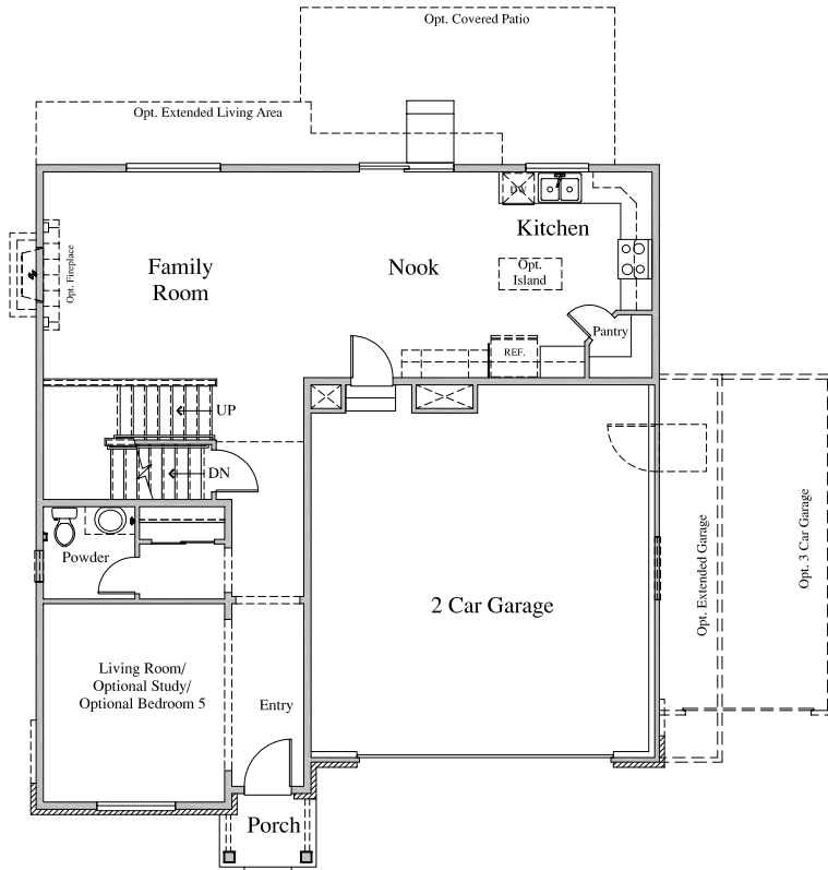
Main Level Plan C21A
